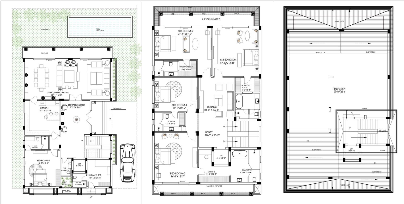
GROUND
