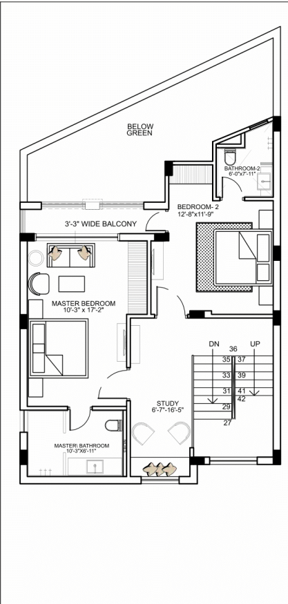
FIRST
