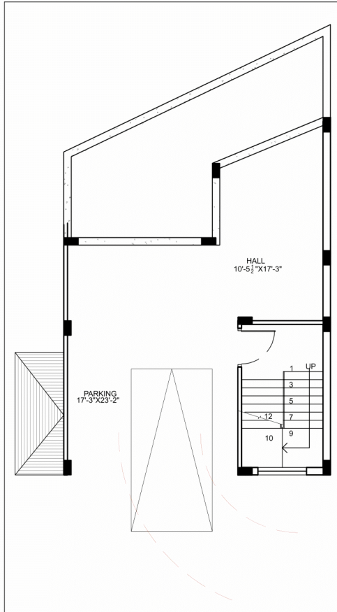
STILT
