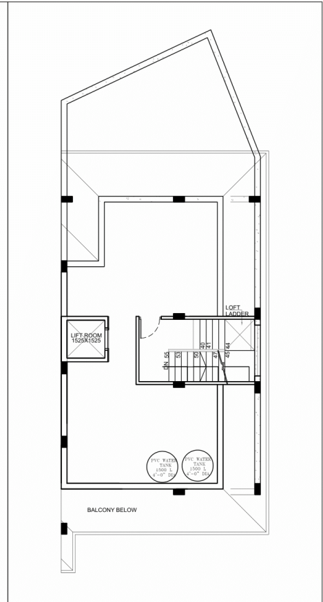
TERRACE
